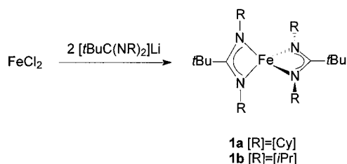
Scheme 1. Formation of the bis(amidinate) iron(II) complexes
